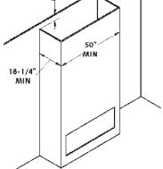
Open chase framing with enclosure min 1-1/4" below ceiling
