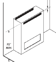
Minimum enclosure with front and back vents
